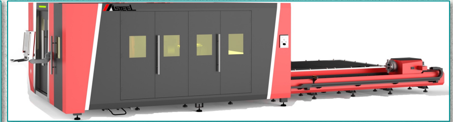
MF-3015TDE sheet / tube fiber laser centre with 3m X-axis x 1.5m Y-axis 20 to 210mm diameter round / 20 to 150mm square x 20' long tube size and a choice of a 2/3/6/12kW laser system
