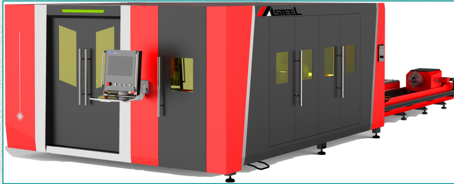
MF-3015TDE sheet / tube fiber laser centre with 3m X-axis x 1.5m Y-axis 20 to 210mm diameter round / 20 to 150mm square x 20' long tube size and a choice of a 2/3/6/12kW laser system
